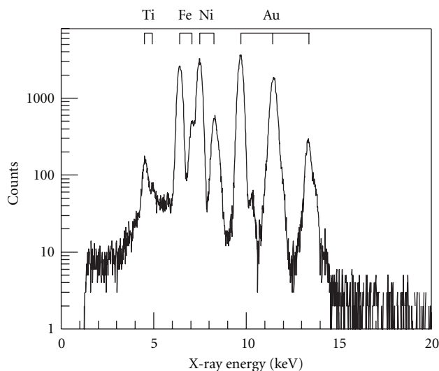
FIGURE 1: A PIXE spectrum of a NiFe thin film deposited from a 100 mM NiSO 4 , 10 mM FeSO 4 , 0.5 M H 3 BO 3 , and 1 M Na 2 SO 4 solution at -900 mV for 6 min. Approximately 1.8 μC of 3.4 MeV protons were incident on the sample to obtain this spectrum. The peaks corresponding to the K X-rays of Ti, Fe, and Ni, and the L X-rays of Au are indicated.
